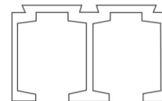
AST 44-03 Track for Double Glass Door Size : 12 Ft. & 16 Ft. ₹ 650/- (Per Ft.)
